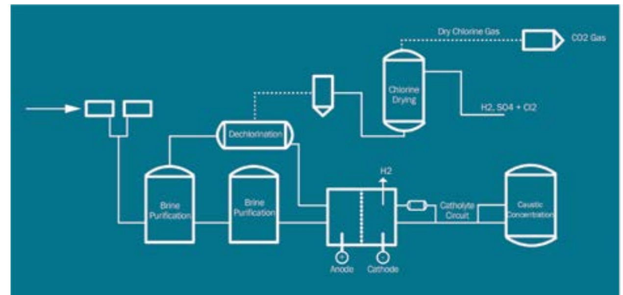
A chlorine production line
